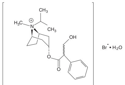
Figure 3. 1-2. Chemical structure of ipratropium bromide.
